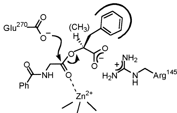
Figure 6. Schematic representation showing a proposed reaction path for the CPA-catalyzed hydrolysis of ester-type substrates, for example, 3 and 4 .
