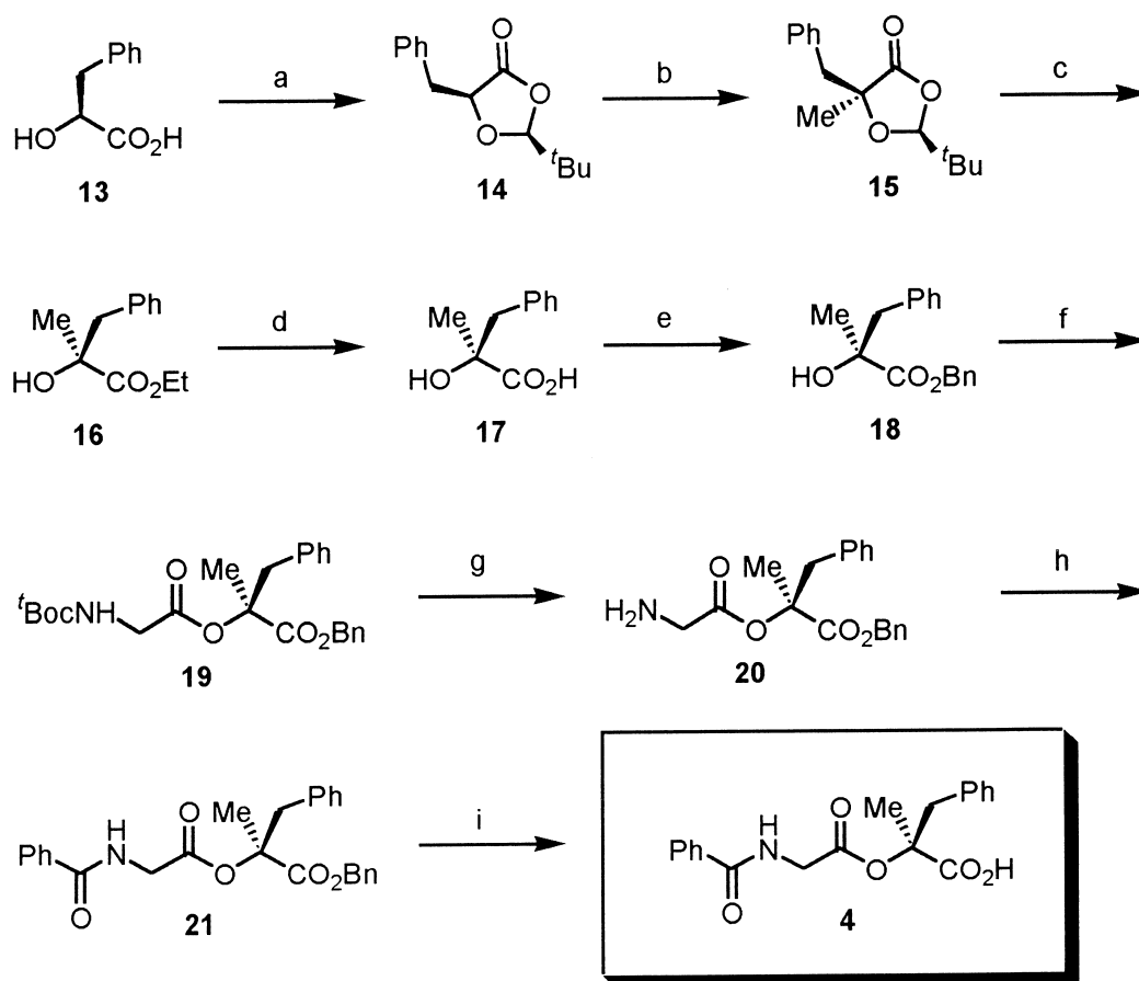
Scheme 3. (a) Pivalaldehyde (1.1 equiv), \text{BF}_3 \cdot \text{Et}_2\text{O} (3 equiv), ether, 0^\circ\text{C} , 4 h, 94%; (b) LDA (1.05 equiv), MeI (1.5 equiv), THF:hexane (9:1), -78^\circ\text{C} to -20^\circ\text{C} , 3 h, 47%; (c) NaOEt (cat.), EtOH, reflux, 10 min, 66%; (d) LiOH·H 2 O (3 equiv), THF:MeOH:H 2 O (3:1:1), rt, 12 h, 96%; (e) \text{Cs}_2\text{CO}_3 (1 equiv), MeOH, rt, 30 min; BnBr (1 equiv), DMF, rt, 6 h, 86%; (f) t Boc-Gly-OH (3 equiv), \text{Sc}(\text{OTf})_3 (0.6 equiv), DMAP (3 equiv), rt, -10^\circ\text{C} , 30 min; EDCI (3 equiv), \text{CH}_2\text{Cl}_2 , -10 to 40^\circ\text{C} , 48 h, 62%; (g) \text{CF}_3\text{CO}_2\text{H} , rt, 1 h, 90%; (h) BzCl (1 equiv), \text{Et}_3\text{N} (1 equiv), \text{CH}_2\text{Cl}_2 , 0^\circ\text{C} to rt, 1 h, 91%; (i) Pd/C, \text{H}_2 , MeOH, rt, 1 h, 95%.
