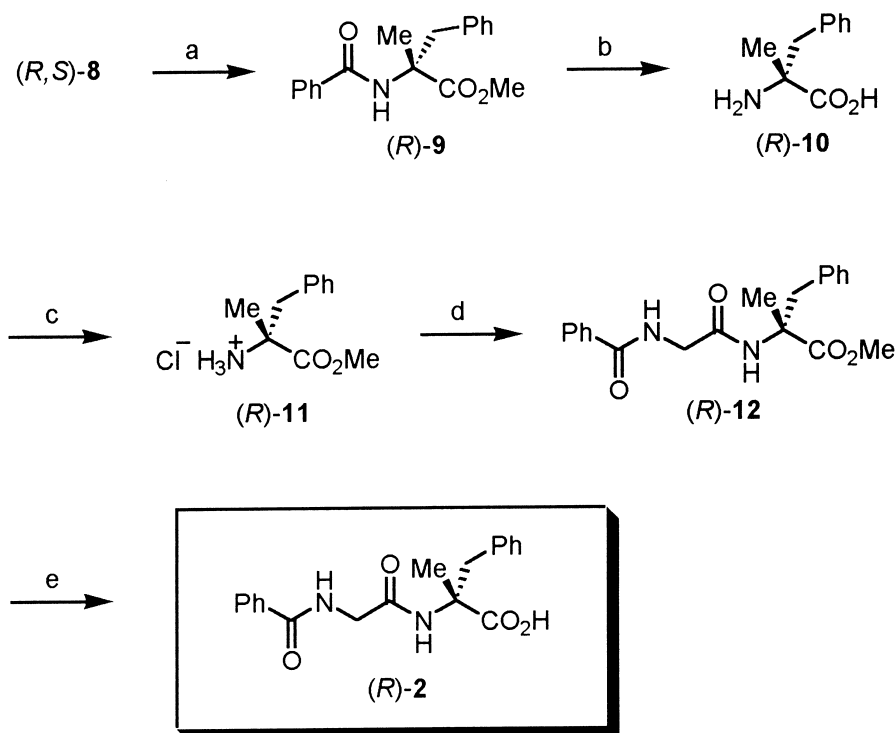
Scheme 2. (a) \text{CF}_3\text{SO}_3\text{H} , MeOH, 80^\circ\text{C} , 20 h, 70%; (b) HCl/dioxane, 100^\circ\text{C} , 20 h; propylene oxide, EtOH, reflux, 0.5 h, 90%; (c) \text{H}^+ , MeOH, reflux, 12 h, 90%; (d) hippuric acid, NMM, isobutyl chloroformate, THF, -10^\circ\text{C} to rt, 12 h, 52%; (e) LiOH·H 2 O (3 equiv), MeOH/H 2 O/THF, rt, 24 h, 90%.
