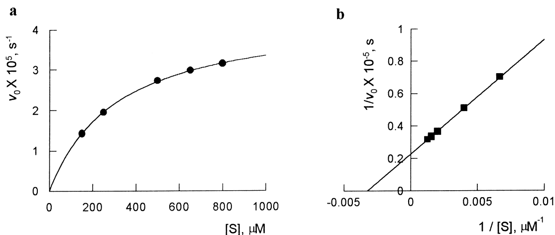
Figure 1. The progress curve (a) and the Lineweaver–Burk plot (b) for CPA catalyzed hydrolysis of ( S )-Hipp- \alpha -MePhe (Tris buffer of pH 7.5 at 25^\circ\text{C} ).
