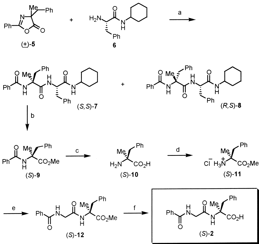
Scheme 1. (a) NMP, 70 °C, 24 h, ( S,S )-7, 39%; ( R,S )-8, 38%; (b) CF 3 SO 3 H, MeOH, 80 °C, 20 h, 70%; (c) HCl/dioxane, 100 °C, 20 h; propylene oxide, EtOH, reflux, 0.5 h, 90%; (d) H + , MeOH, reflux, 12 h, 90%; (e) hippuric acid, NMM, isobutyl chloroformate, THF, −10 °C to rt, 12 h, 52%; (f) LiOH·H 2 O (3 equiv), MeOH/H 2 O/THF, rt, 24 h, 90%.
