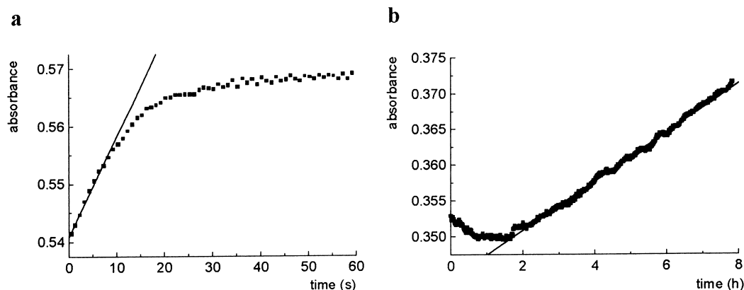
Figure 2. Graphs showing the product formation against time for CPA catalyzed hydrolysis of (S)-Hipp-Phe (a) and (R)-Hipp- \alpha -MePhe (b) at [S] = 250 \mu\text{M} and [CPA] = 600 nM (Tris buffer of pH 7.5 at 25 °C).
