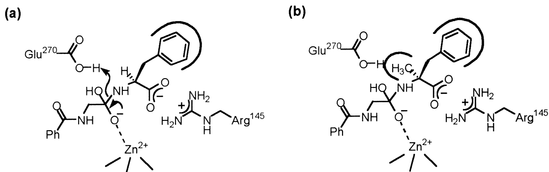
Figure 5. Schematic representations showing the tetrahedral transition state proposed for the CPA-catalyzed hydrolysis of normal peptide substrate ( 1 ) (a) and unnatural substrate ( 2 ) whose \text{P}_1' residue carries a methyl group at the \alpha -position.
