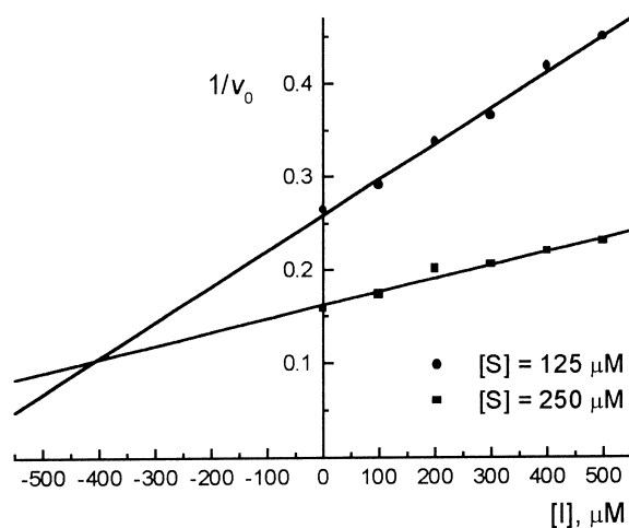
Figure 3. The Dixon plot 10 for the inhibition of the CPA catalyzed hydrolysis of (S)-Hipp-Phe by (R)-Hipp- \alpha -MePhe (Tris buffer of pH 7.5 at 25 °C).
